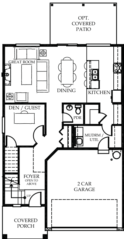
Main Floor
