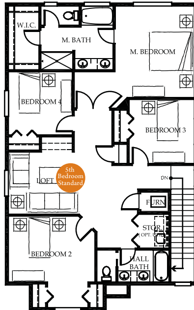
Upper Floor
