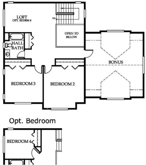
Upper Floor
