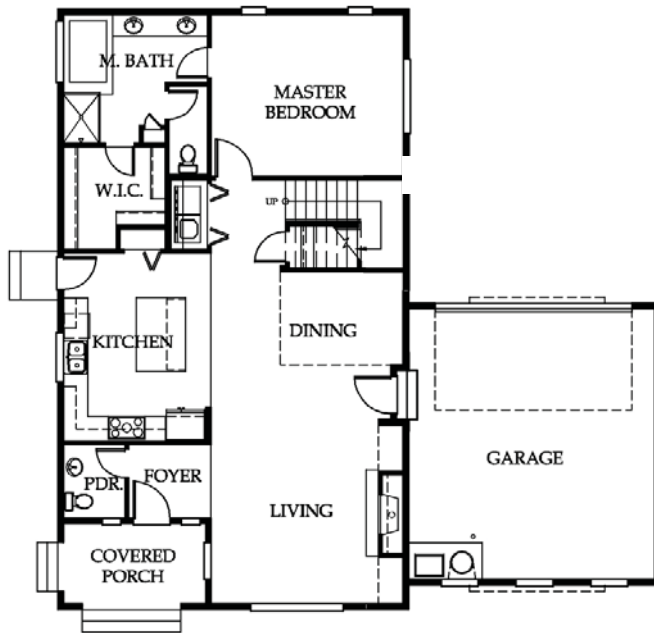
Main Floor
